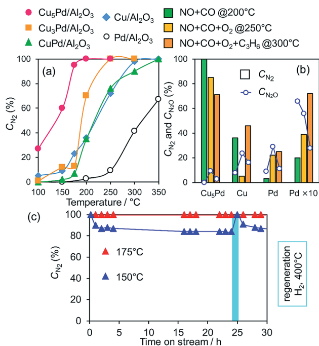
Fig. 3 (a) NO conversion to N_2 during the NO reduction by CO over Pd, Cu, and Cu–Pd catalysts as a function of reaction temperature (NO, CO: 0.5%, GHSV = 80 000 h -1 ). (b) Comparison between C_{N_2} and C_{N_2O} in NO reduction in the presence of O_2 and C_3H_6 . (c) Stability test for Cu_5Pd/Al_2O_3 in the NO + CO reaction at low temperatures (NO, CO: 0.5%, GHSV = 40 000 h -1 ).
