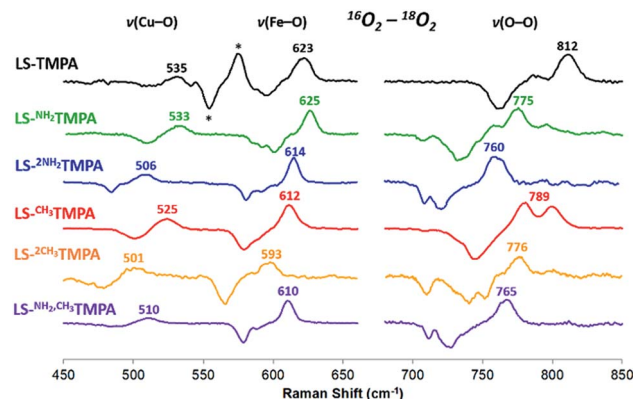
Fig. 8 Comparison of rR data ( ^{16}\text{O}_2 – ^{18}\text{O}_2 ) for the \text{LS-XTMPA} complexes, which are normalized to equal \nu(\text{Fe}-\text{O}) and \nu(\text{O}-\text{O}) intensities to aid in visual comparison. Isotope-sensitive features are labelled by their frequency in ^{16}\text{O}_2 . Note that some modes (e.g. 789 \text{cm}^{-1} in red spectrum) are split by Fermi coupling. Asterisks (*) denote a ferric superoxo impurity. Laser excitation was 413 nm or 780–890 nm, see ESI.†
