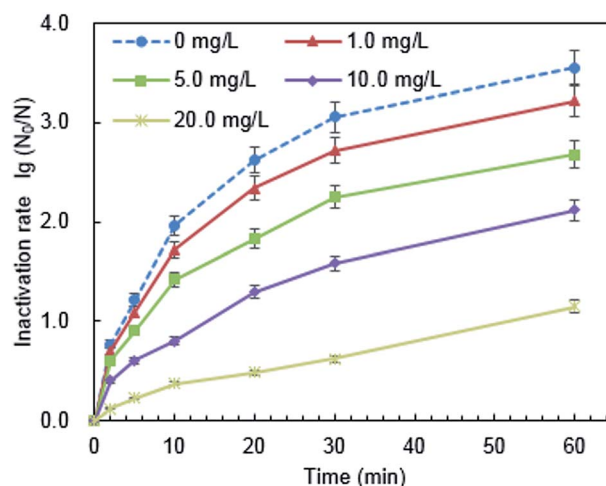
Fig. 9 Effect of HA on antibacterial efficacy to B. subtilis with PQAS-AgNPs. Reaction conditions: [\text{AgNPs}] = 10.0 \text{ mg L}^{-1} , reaction time = 60 min, pH = 7.1, T = 25^\circ\text{C} , initial concentration of B. subtilis : 10^6 \text{ CFU mL}^{-1} .
