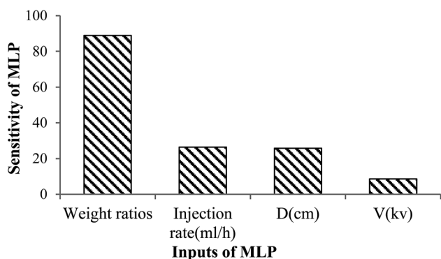
Fig. 9 Sensitivity analysis of PDFNF MLP .
