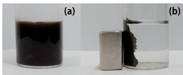
Fig. 9 A reaction mixture in the absence (a) or presence (b) of a magnetic field.
