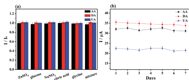
Fig. 7 (a) Peak current ratio of MoS 2 -PANI/rGO/GCE to 1.0 mM AA, 75 \mu\text{M} DA, and 75 \mu\text{M} UA in the presence of 1 mM of various interfering substances (ZnSO 4 , glucose, NaNO 3 , citric acid, glycine, and the mixture, respectively). (b) The stability of MoS 2 -PANI/rGO/GCE in 0.1 M PBS (pH 7.0, 0.1 M KCl) containing 1.0 mM AA, 75 \mu\text{M} DA, and 75 \mu\text{M} UA.
