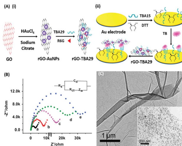
Fig. 15 (A) Schematic illustration of (i) synthesis of rGO-AuNPs-apptamer conjugates and (ii) development of a signal amplified impedimetric aptasensing platform for thrombin (TB) detection. (B) EIS responses of the developed platform for various concentrations of thrombin. Inset shows the Randles-Sevcik circuit diagram applied to obtain Nyquist plots. (C) Transmission electron micrographs showing rGO and the rGO-AuNP conjugate (inset). Adapted with permission from ref. 131. Copyright (2015) Elsevier.
