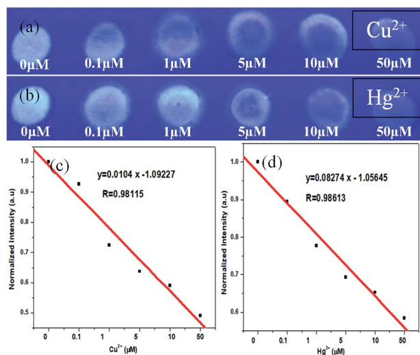
Fig. 9 Digital photograph, under 365 nm UV lamp, of NCDs in circular reaction pots on interaction with different concentrations (0.1 μM to 50 μM) of (a) Cu 2+ and (b) Hg 2+ . Fluorescence intensity versus metal ion concentration plot (c) corresponding to (a) and (d) corresponding to (b) (fluorescence intensity of the filter paper loaded NCDs with an increase in concentration of Cu 2+ or Hg 2+ ions, analysed with ImageJ software).
