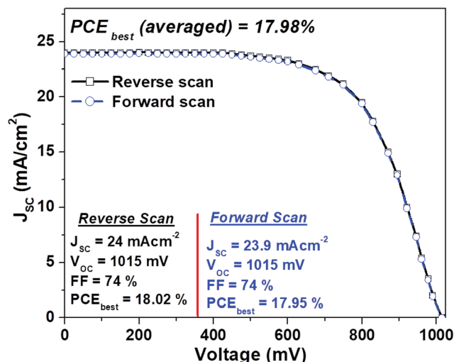
Fig. 5 J - V curves (both in the forward and reverse scans) for the best-performing device with MAPbI 3 micro-needles.
