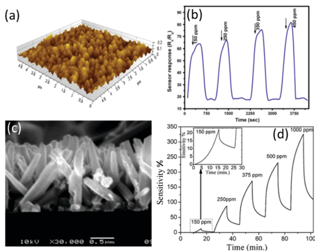
Fig. 8 (a) AFM image of the ZnO films and (b) response/recovery curves of a ZnO film-based gas sensor to different concentrations of H 2 . 189 Copyright 2014, Springer Nature. (c) Cross section SEM image of the ZnO nanorods and (d) response/recovery curves of a ZnO nanorod-based gas sensor to different concentrations of H 2 . 191 Copyright 2013, Elsevier.
