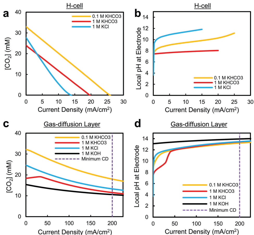
Fig. 3 Simplified predictions of the electrode concentration of CO 2 and pH for commonly-used electrolytes as a function of current density in an (a and b) H-cell with a 50 μm CO 2 diffusion thickness and, (c and d) a gas-diffusion layer with a 50 nm CO 2 diffusion thickness and liquid diffusion layer of 200 μm. A Faradaic efficiency of CO 2 -to-CO of 90% is assumed.
