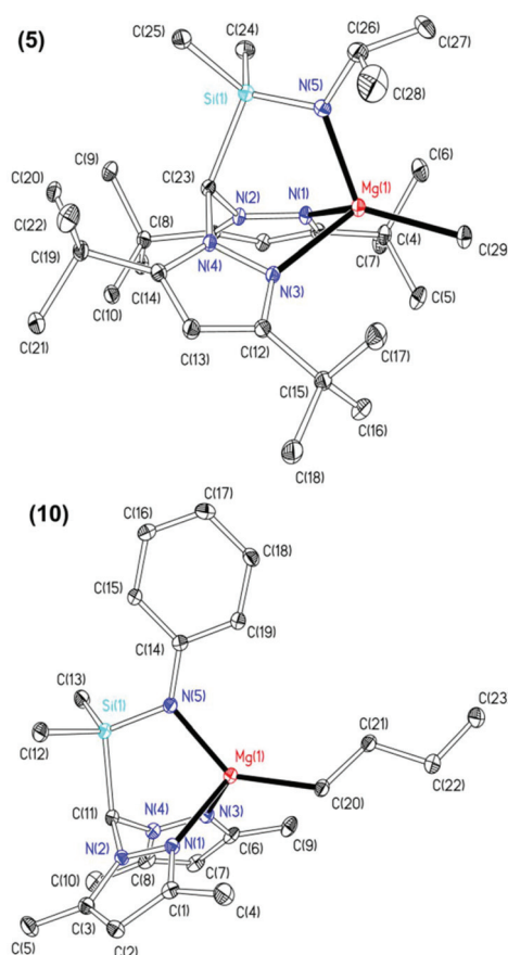
Fig. 1 Thermal displacement ellipsoid drawings (20% probability ellipsoids) of \text{Mg}\{\text{HC}(t\text{Bu}_2\text{pz})_2\text{SiMe}_2\text{N}^i\text{Pr}\}\text{Me} ( 5 , top) and \text{Mg}\{\text{HC}(\text{Me}_2\text{pz})_2\text{SiMe}_2\text{NPh}\}^n\text{Bu} ( 10 , bottom). All hydrogen atoms have been omitted for clarity.
