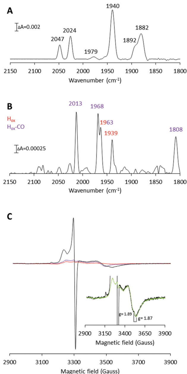
Fig. 4 H-Cluster assembly monitored by FTIR and X-band EPR spectroscopy. (A) FTIR spectrum recorded on 2.5 mM [2Fe] ad -CaHydF (reproduced from Fig. 2, panel B). (B) FTIR spectrum recorded on a mixture of apo-CrHydA1 (1.5 mM) and [2Fe] ad -CaHydF (300 \mu M) after 60 min incubation in 25 mM Tris-HCl pH 7.0, 50 mM KCl. Color coding: H ox , red; H ox -CO, purple. (C) X-band EPR spectra. Black line: apo-CrHydA1 (200 \mu M) incubated with [2Fe] ad -CaHydF (30 \mu M) for 60 min; Red line: [2Fe] ad -CaHydF (30 \mu M); Purple line: apo-CrHydA1 (200 \mu M). (Inset): Black line: apo-CrHydA1 (200 \mu M) treated with [2Fe] ad -CaHydF (30 \mu M); Green line: a linear combination of [4Fe4S] + -CaHydF (16 \mu M) and apo-CrHydA1 (200 \mu M). All EPR samples were prepared in 100 mM Tris-HCl pH 7.0 300 mM KCl, and recorded at a microwave power of 1 mW, at 10 K, microwave frequency: 9.28 GHz.
