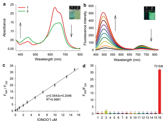
Fig. 2 (a) Absorption spectra of Gal-NIR (5 \mu M) in the absence (1) and presence (2) of ONOO - (15 \mu M). Inset: The corresponding color image. (b) Fluorescence spectra of Gal-NIR (5 \mu M) upon adding various amounts of ONOO - (0, 0.5, 1.0, 2.0, 3.0, 5.0, 7.0, 10.0, 13.0, and 15.0 \mu M) in PBS buffer solution (pH 7.4). \lambda_{\text{ex}} = 440 nm. Inset: Corresponding fluorescence image under 365 nm ultraviolet radiation. (c) The fluorescence intensity ratio ( F_{500}/F_{720} ) versus ONOO - concentration. (d) The fluorescence intensity ratio to ONOO - (15 \mu M) and other various analytes (150 \mu M). 1: blank, 2: ClO - , 3: H 2 O 2 , 4: ROO • , 5: O 2 - , 6: ·OH, 7: NO, 8: NO 2 - , 9: NO 3 - , 10: H 2 S, 11: SO 3 2- , 12: HSO 3 - , 13: Cys, 14: Hcy, 15: GSH, and 16: ONOO - .
