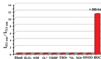
Fig. 75 Fluorescence responses ( I_{511\text{nm}}/I_{713\text{nm}} ) of probe 51 (5 \mu M) toward HOCl (10 \mu M) and other ROS (100 \mu M) in PBS (10 mM) solution (ethanol/water = 1/1, v/v, pH 7.4); \lambda_{\text{ex}} = 480 nm, 635 nm. Copyright 2017 Elsevier.
