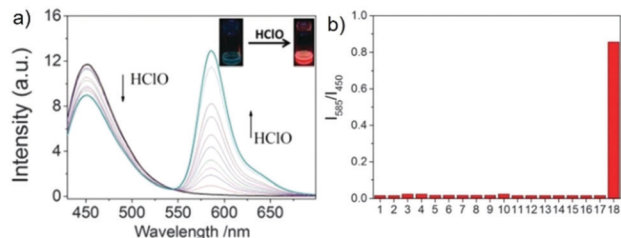
Fig. 72 (a) Emission spectra (excitation at 420 nm) of probe 50 (10 \mu M) in the presence of various amounts of NaOCl (0 to 80 \mu M) in PBS buffer (pH 5.0, containing 30% DMSO as a cosolvent). The inset shows the visual fluorescence color of the chemodosimeter 50 (20 \mu M) before (left) and after (right) the addition of 50 \mu M of HOCl upon excitation at 365 nm using a hand-held UV lamp. (b) Ratios of fluorescence intensity ( I_{585}/I_{450} ) of probe 50 (5.0 \mu M) to various relevant species (100 \mu M): (1) blank; (2) \text{Co}^{2+} ; (3) \text{Cu}^{2+} ; (4) \text{Ni}^{2+} ; (5) \text{Br}^- ; (6) \text{I}^- ; (7) \text{NO}_2^- ; (8) \text{NO}_3^{2-} ; (9) \text{OH}^- ; (10) \text{S}^{2-} ; (11) Cys; (12) GHS; (13) Hcy; (14) t -butylhydroperoxide; (15) peroxide tert -butyl ether; (16) \text{H}_2\text{O}_2 ; (17) NO and (18) HOCl in pH 5.0 PBS buffer (30% DMF as a cosolvent). Copyright 2016 Royal Society of Chemistry.
