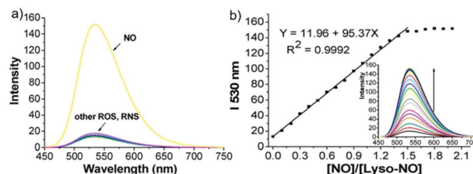
Fig. 102 (a) Selectivity of 63 (11 \mu M) fluorescence response for NO over other reactive nitrogen and oxygen species (5.0 equiv.) in 20 : 80 CH 3 CN–H 2 O solution at pH 5.0 (in 10 mM phosphate buffer). (b) Intensity at 530 nm vs. NO concentration under the same conditions. Inset: Changes in fluorescence spectra of 63 (11 \mu M) upon addition of different amounts NO solution (0–2.0 equiv.). Copyright 2012 American Chemical Society.
