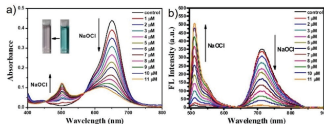
Fig. 74 (a) UV-vis spectra of probe 51 (5 \mu M) upon addition of NaOCl (0–10 \mu M) in PBS (10 mM) solution (ethanol/water = 1/1, v/v, pH 7.4). Inset: The color of probe 51 (5 \mu M) in the absence and presence of NaOCl (10 \mu M). (b) Fluorescence emission of probe 51 (5 \mu M) upon the addition of increasing concentrations of NaOCl in PBS (10 mM) solution (ethanol/water = 1/1, v/v, pH 7.4). Copyright 2017 Elsevier.
