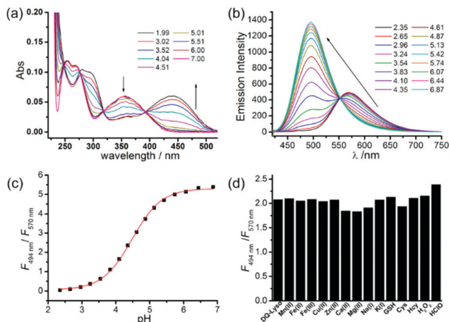
Fig. 44 (a) Absorption spectra of probe 29 (5 \mu\text{M} ). (b) Fluorescence spectra of probe 29 (2 \mu\text{M} ) in \text{Na}_2\text{HPO}_4 -citrate buffer (10 mM \text{Na}_2\text{HPO}_4 and 10 mM citric acid) at various pH values. (c) Ratio ( F_{494\text{nm}}/F_{570\text{nm}} ) changes as a function of the pH values. (d) Emission spectra of probe 29 (2 \mu\text{M} ) in the presence of various metal ions (100 \mu\text{M} \text{Mn}^{2+} , \text{Fe}^{3+} , \text{Fe}^{2+} , \text{Cu}^{2+} , \text{Zn}^{2+} , and 1 mM \text{Mg}^{2+} , \text{Ca}^{2+} , \text{Na}^+ , and \text{K}^+ ), 5 mM thiols (GSH, Cys, Hcy), and 100 \mu\text{M} \text{H}_2\text{O}_2 and \text{NaClO} in \text{Na}_2\text{HPO}_4 -citrate buffer (pH = 4.2); \lambda_{\text{ex}} = 405 nm. Copyright 2013 American Chemical Society.
