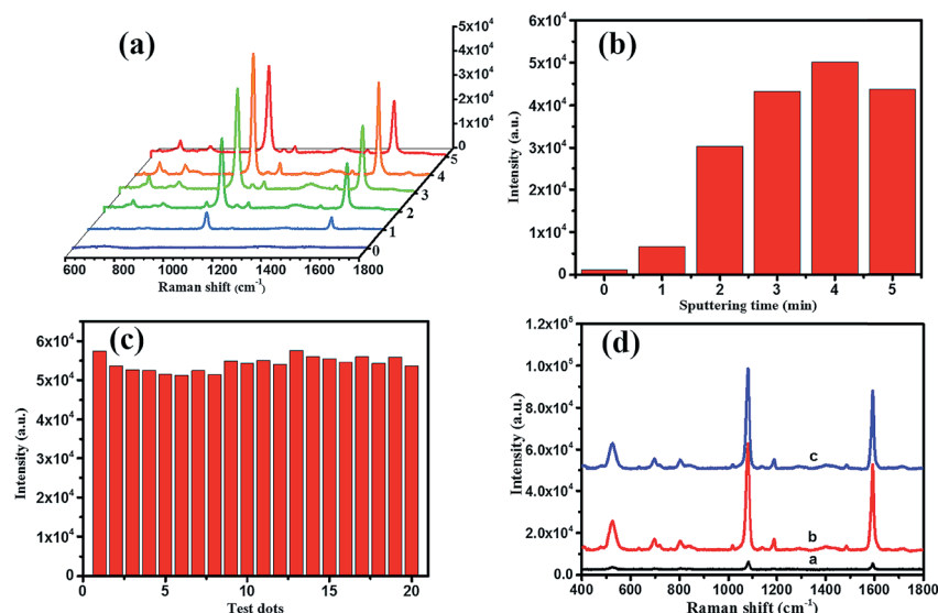
Fig. 6 (a) SERS spectra and (b) the intensities of SERS peaks at 1078 cm -1 of 4MBA (10 mM) dropped on the surfaces of Ag/TiO 2 NWs substrates prepared at different sputtering times; (c) the intensities of the SERS peak at 1078 cm -1 collected from 20 random testing spots on the optimal SERS-active substrate; (d) Raman spectra of 4MBA powder on a quartz slide (line a), the freshly prepared substrate (line b) and the saved substrate (line c).
