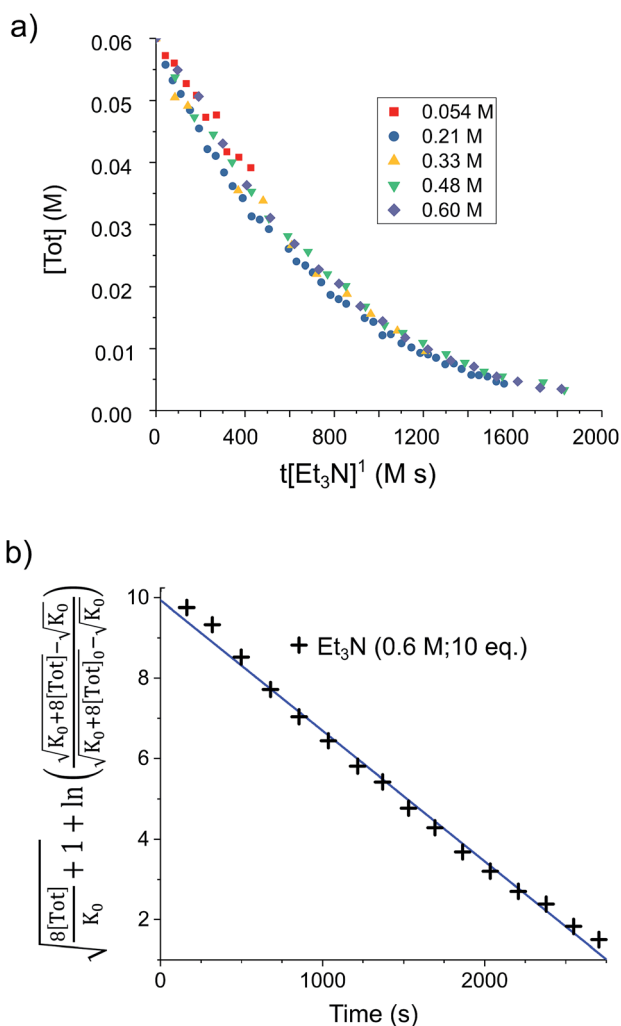
Fig. 3 (a) Solutions of 1 (0.03 mmol) in d_8 -toluene (0.5 mL) under \text{H}_2 (4 bar) containing various base concentrations were prepared. When the stannylenic concentration, [\text{Tot}] , is plotted against the normalised timescale t \cdot [\text{Et}_3\text{N}]^1 , all traces overlap, confirming the order in base to be one. (b) Linearised rate data for a similar solution of 1 (0.03 mmol) in d_8 -toluene (0.5 mL) under \text{H}_2 (4 bar) containing \text{Et}_3\text{N} (0.6 M; 10 eq.).
