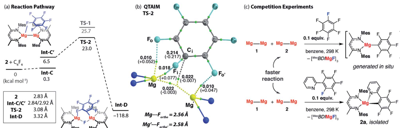
Fig. 6 (a) The calculated reaction pathway for C–F activation with 2, inset shows Mg...Mg separation. (b) QTAIM plot of TS-2: \rho_{(r)} values in bold, \nabla^2\rho values in parentheses. Full QTAIM for TS-2 in Fig. S31†. (c) Competition experiments between 1 or 2 and fluoroarenes.
