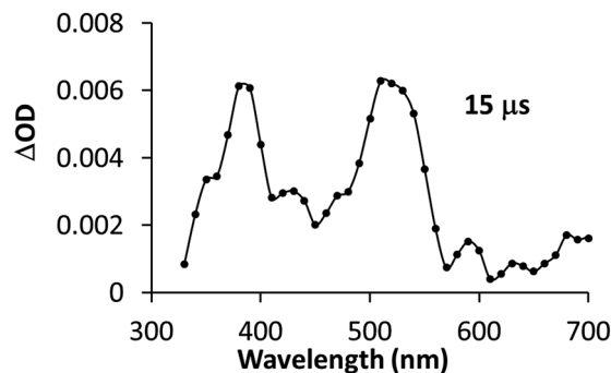
Fig. 9 Transient absorption spectrum of a solution containing \text{PS}_{\text{Ir}}^+ (50 \mu\text{M} ), \text{Et}_3\text{N} (20 mM) and \mathbf{1}^{\text{CO2Et}} (80 \mu\text{M} ) recorded at 15 \mu\text{s} after laser excitation. All measurements were carried out under \text{N}_2 at room temperature in acetonitrile ( \lambda_{\text{ex}} = 355 nm, E = 8 mJ per pulse).
