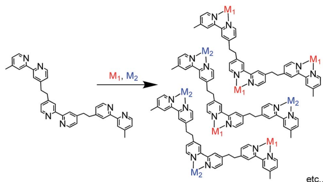
Scheme 1 Difficulty of the conventional method for synthesising trinuclear complexes with trisdiamine bridging ligands.
