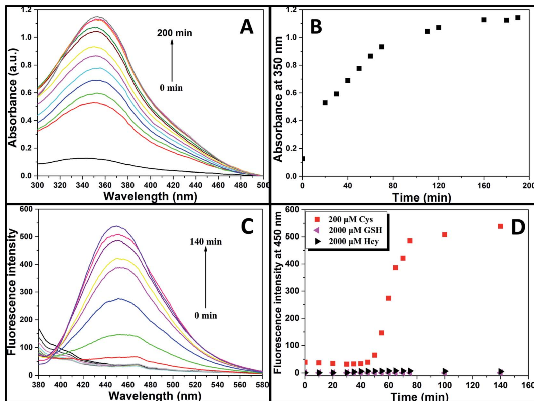
Fig. 2 (A) UV-vis spectra, (B) dependence of absorbance intensity at 350 nm with time, and (C) fluorescent spectra of TPE-NP solution (240 \mu M in PBS/DMSO ( v/v = 8/2 ), pH = 7.4) in the presence of Cys (200 \mu M). (D) The time course of the fluorescence intensity at 450 nm of TPE-NP solution (240 \mu M in PBS/DMSO ( v/v = 8/2 ), pH = 7.4) in the presence of 200 \mu M Cys and 2000 \mu M of Hcy and GSH.
