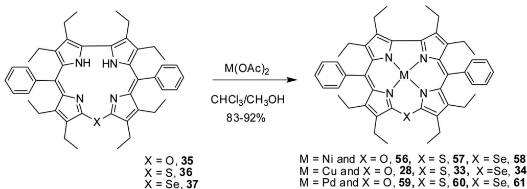
Scheme 15 Synthesis of Cu(II) ( 28 , 33 , 34 ) Ni(II) ( 56–58 ), and Pd(II) ( 59–61 ) complexes of 10-heterocorrole 35–37 .
