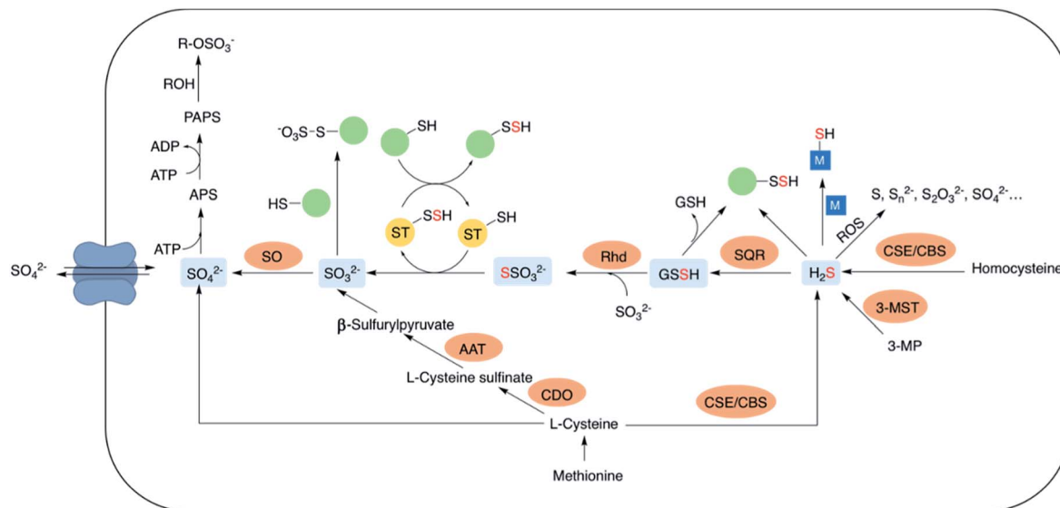
Fig. 2 A partial ensemble of sulfur oxidation states and their distinct physiological roles. CBS: cystathionine-β-synthase; CSE: cystathionine-γ-lyase; 3-MST: 3-mercaptopyruvate sulfurtransferase; SQR: sulfide quinone oxidoreductase; Rhd: rhodanese; SO: sulfite oxidase; AAT: aspartate aminotransferase; CDO: cysteine dioxygenase; APS: adenosine-5'-phosphosulfate; PAPS: 3'-phosphoadenosine-5'-phosphosulfate.
