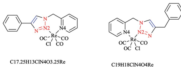
\text{C}_{19}\text{H}_{18}\text{ClN}_4\text{O}_4\text{Re}
