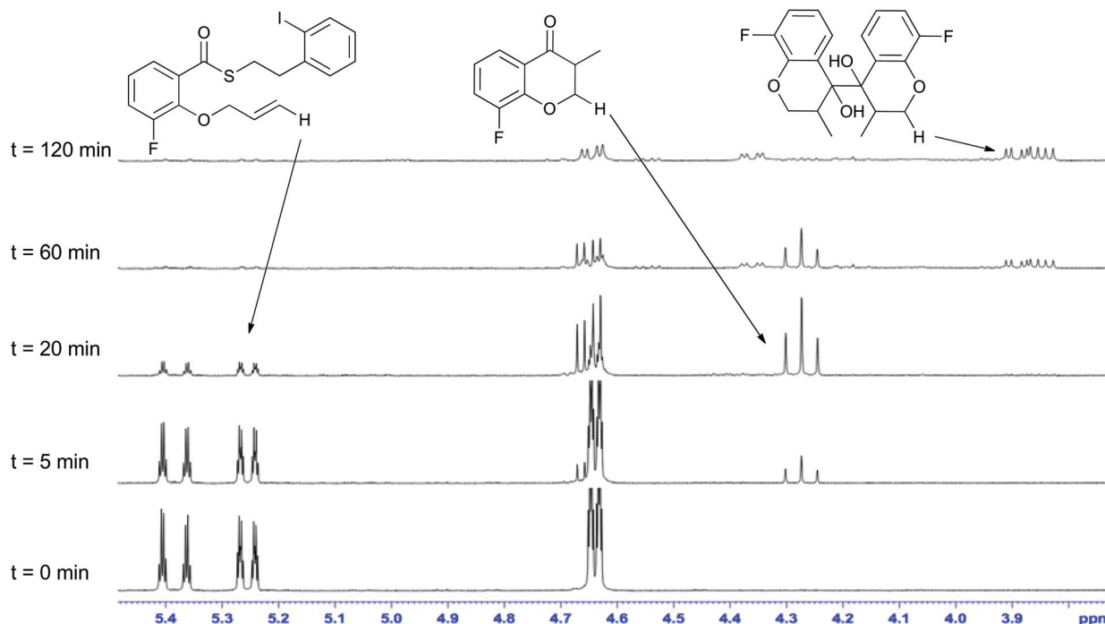
Fig. 1 In situ ^1\text{H} NMR analysis of the dimerization reaction mixture.
