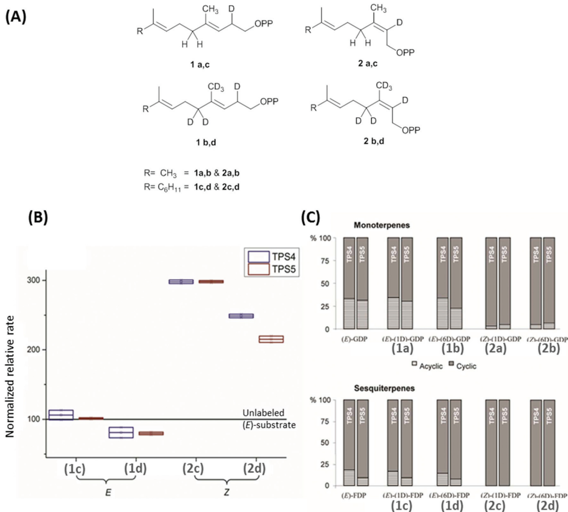
Fig. 4 (A) Monodeuterated and hexadeuterated ( 2E -GDP, ( 2E -FDP (1a–d) and ( 2Z -GDP, ( 2Z -FDP (2a–d) used for isotope sensitive branching studies. (B) Comparison of total rates of sesquiterpene formation and (C) ratio acyclic/cyclic volatile formation with the incubation of deuterated ( E )/( Z )-GDP and ( E )/( Z )-FDP with TPS4 and TPS5. (B) Comparison of relative rates of sesquiterpene volatile formation from monodeuterated substrates (1c, 2c) and hexadeuterated substrates (1d, 2d). Volatile production improved by \sim 200\% and \sim 150\% with the mono and hexadeuterated substrate on comparison with unlabelled substrate (baseline at 100). (C) There was a distinct absence of acyclic products in the substrate with ( 2Z )-substrates seen in both monoterpenes (2a, 2b) and sesquiterpenes (2c, 2d). 100
