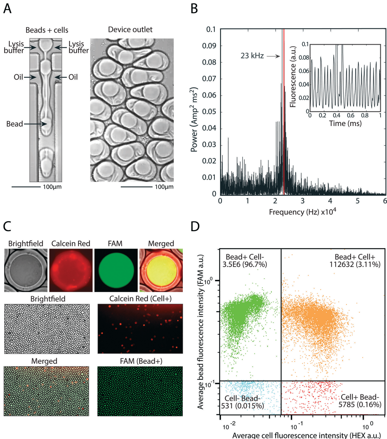
Fig. 5 Pairing cells with beads at 23 kHz. A) Device operation and the resultant droplets in the outlet. B) Power spectrum of fluorescent time trace data (inset) used to calculate drop making frequency. C) Fluorescence microscopy of FAM-stained beads and calcein red cells demonstrates bead loading and cell-bead pairing. D) High throughput analysis of millions of bead-containing droplets and hundreds of thousands of bead-cell pairings using a droplet cytometer.
