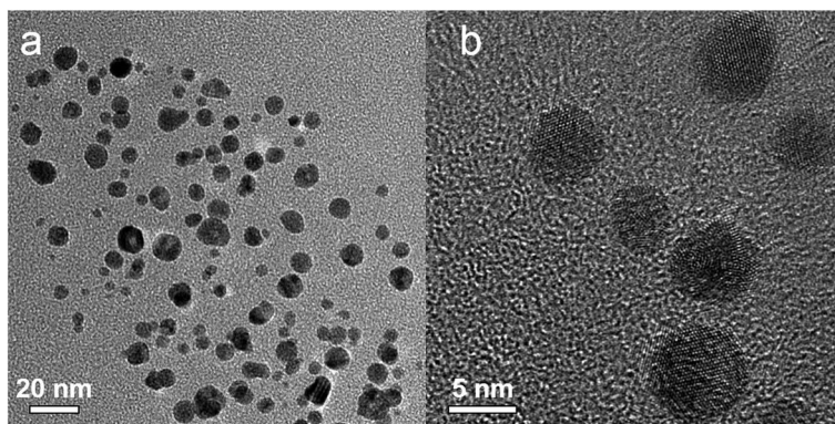
Fig. 10 (a) TEM and (b) HRTEM images of nanoparticles synthesised using only \text{Pd}(\text{NO}_3)_2 in Reactor 3 and HQ in Reactor 4.
