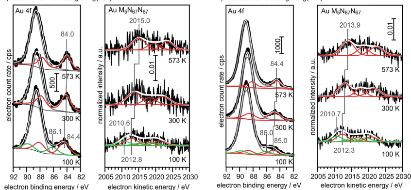
Fig. 7 XPS and X-ray excited Auger spectra of 0.02 ML Au/30 ML MgO (a) and 0.02 ML Au/3 ML MgO (b) for different annealing temperatures (bottom: 100 K; middle: 300 K; top: 573 K).
