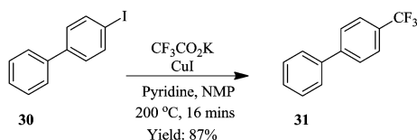
Scheme 9 Continuous flow trifluoromethylation using potassium trifluoroacetate as CF 3 source.
