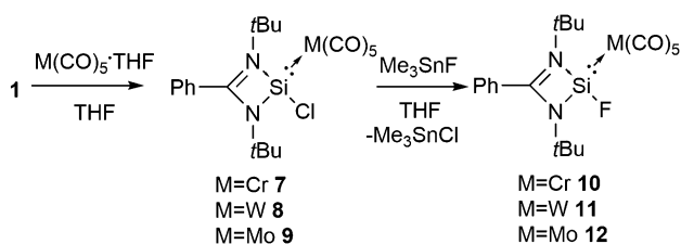
Scheme 3 The synthesis of amidinato stabilized Si(IV) fluorides in the coordination sphere of transition metals.
