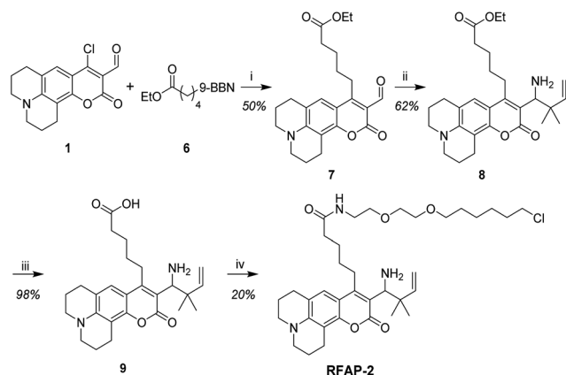
Scheme 5 Synthesis of RFAP-2. Reagents and conditions: (i) Pd-PEPPSI-IPr, \text{K}_3\text{PO}_4 \cdot \text{H}_2\text{O} , THF, rt, 10 h; (ii) \text{NH}_3 , MeOH, 0 ^\circ\text{C} , then prenilyboronic acid, rt, 10 h; (iii) LiOH, THF/MeOH/ \text{H}_2\text{O} , rt, 6 h; (iv) 2-((6-chlorohexyl)oxy)ethan-1-amine, HATU, DIPEA, DMF, rt, 12 h.
