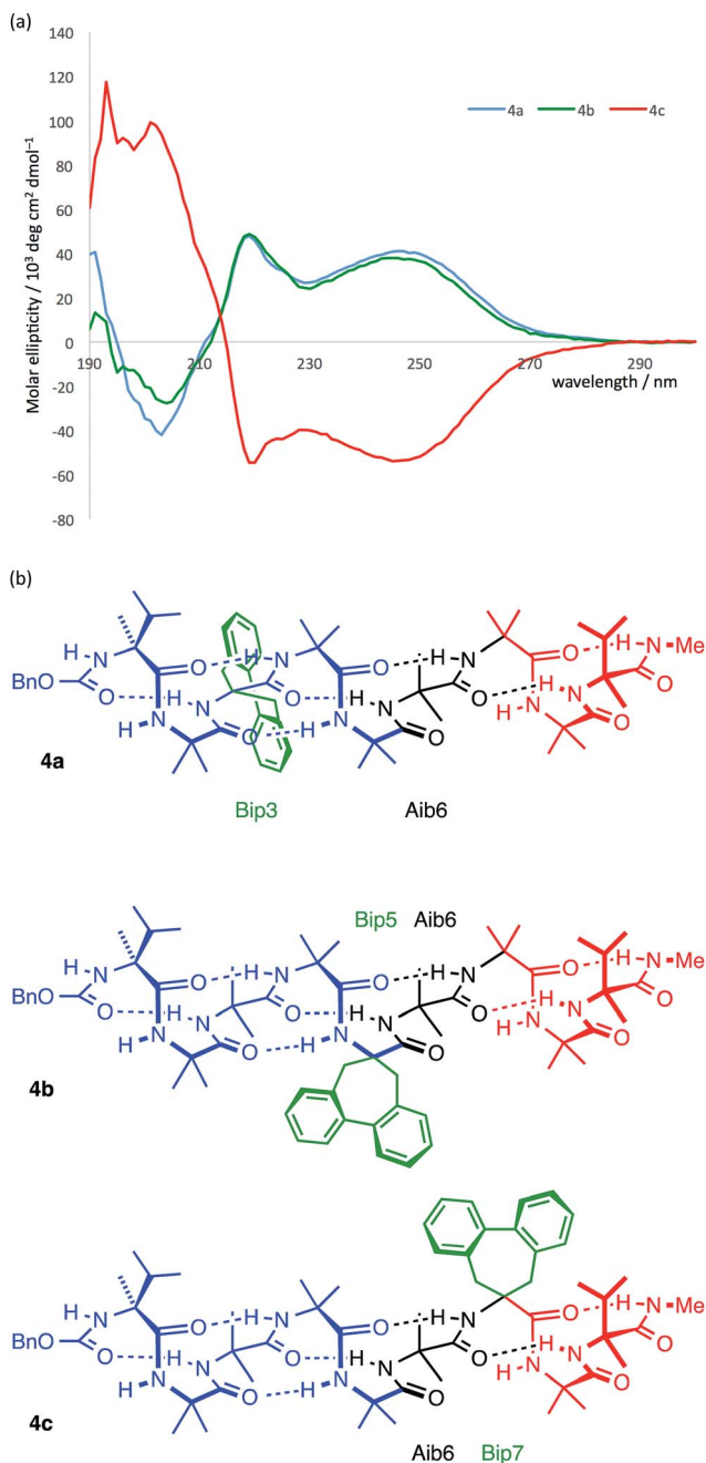
Fig. 9 (a) CD spectra of compounds 4a – c indicating that the Bip residue is in a P environment in 4a and 4b and in an M environment in 4c ; (b) presumed principal conformation of the three isomers, with the screw-sense reversal located at Aib6. Blue indicates right-handed screw sense; red indicates left-handed screw sense.
