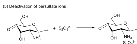
Fig. 2 The proposed mechanism for the degradation of chitosan by KPS free radical. Reproduced from ref. 59. Copyright (2006), with permission from Elsevier.
