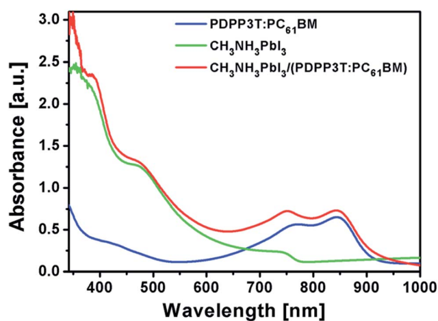
Fig. 26 Comparison of absorption spectra for PDPP3T- \text{PC}_{61}\text{BM} (1 : 2) blend film, \text{CH}_3\text{NH}_3\text{PbI}_3 film, and \text{CH}_3\text{NH}_3\text{PbI}_3/(\text{PDPP3T-PC}_{61}\text{BM}) (1 : 2) bilayer film. 133
