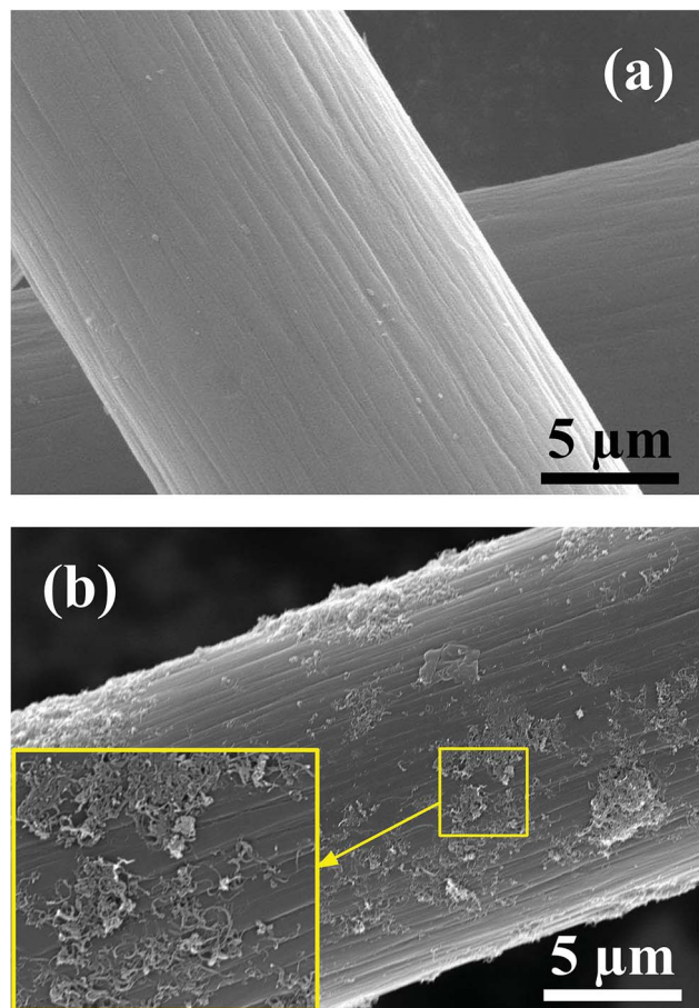
Fig. 5 SEM images of the pristine graphite felt (a) and MWCNTs-NS modified graphite felt (b).
