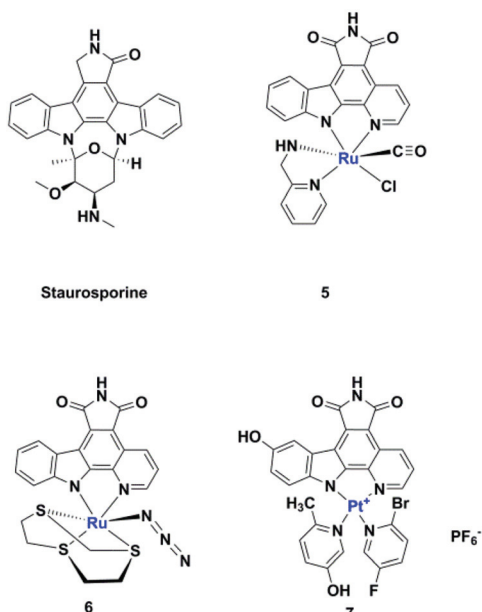
Fig. 2 Staurosporine analogues.
