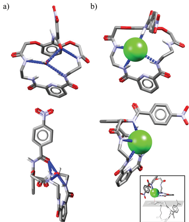
Fig. 8 Crystal structures of the free (a) and chloride complex (b) of the Cr1 .
