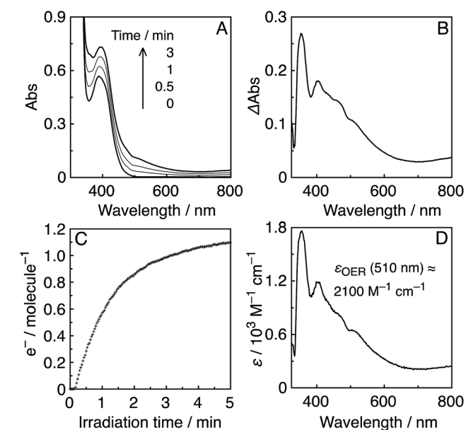
Fig. 4 (A) UV-vis absorption spectral changes of an Ar-saturated DMF-TEOA (5 : 1 v/v) solution containing R(5) (0.05 mM) under irradiation at \lambda_{ex} = 436 nm ( 5.6 \times 10^{-9} einstein per s). (B) Differential absorption spectrum before irradiation and after 3 min irradiation. (C) Time course of accumulated electrons in R(5) , compensated for the inner filter effect. (D) Differential absorption spectrum of R(5) before and after bulk electrolysis in an Ar-saturated DMF solution at -1.95 V vs. Ag/AgNO 3 .
