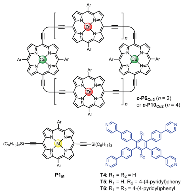
Fig. 1 Chemical structures of the porphyrin nanorings c\text{-P6}_{\text{Cu}_2} ( n = 2 ) and c\text{-P10}_{\text{Cu}_2} ( n = 4 ), \text{P1}_M (where M = \text{Zn}, \text{Cu}, or 2\text{H} ), and the templates T4 , T5 and T6 . Ar = 3,5-bis( tert -butyl)phenyl.
