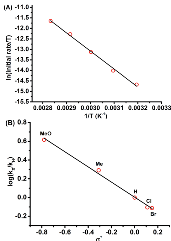
Fig. 1 (A) (top) Plot of ln(initial rate/ T ) vs. 1/T for the reaction between 1a and NFSI in DCE, [ 1a ] = 0.15 M, [NFSI] = 0.1 M, slope = -8.61 \times 10^3 , y-intercept = 1.27 \times 10 , r^2 = 0.996 . (B) (bottom) Hammett plot of log( k_X/k_H ) vs. \sigma^+ for the reaction of NFSI with para substituted diazo phenyl acetates 1 in DCE at 50 °C, [ 1 ] = 0.15 M, [NFSI] = 0.1 M, slope = -0.81 , y-intercept = 0.4 \times 10^{-2} , r^2 = 0.995 .
