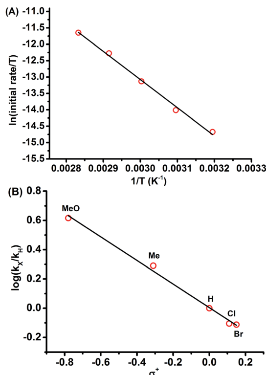
Fig. 1 (A) (top) Plot of ln(initial rate/T) vs. 1/T for the reaction between 1a and NFSI in DCE, [ 1a ] = 0.15 M, [NFSI] = 0.1 M, slope = -8.61 \times 10^3 , y-intercept = 1.27 \times 10 , r^2 = 0.996 . (B) (bottom) Hammett plot of log( k_X/k_H ) vs. \sigma^+ for the reaction of NFSI with para substituted diazo phenyl acetates 1 in DCE at 50 °C, [ 1 ] = 0.15 M, [NFSI] = 0.1 M, slope = -0.81 , y-intercept = 0.4 \times 10^{-2} , r^2 = 0.995 .
