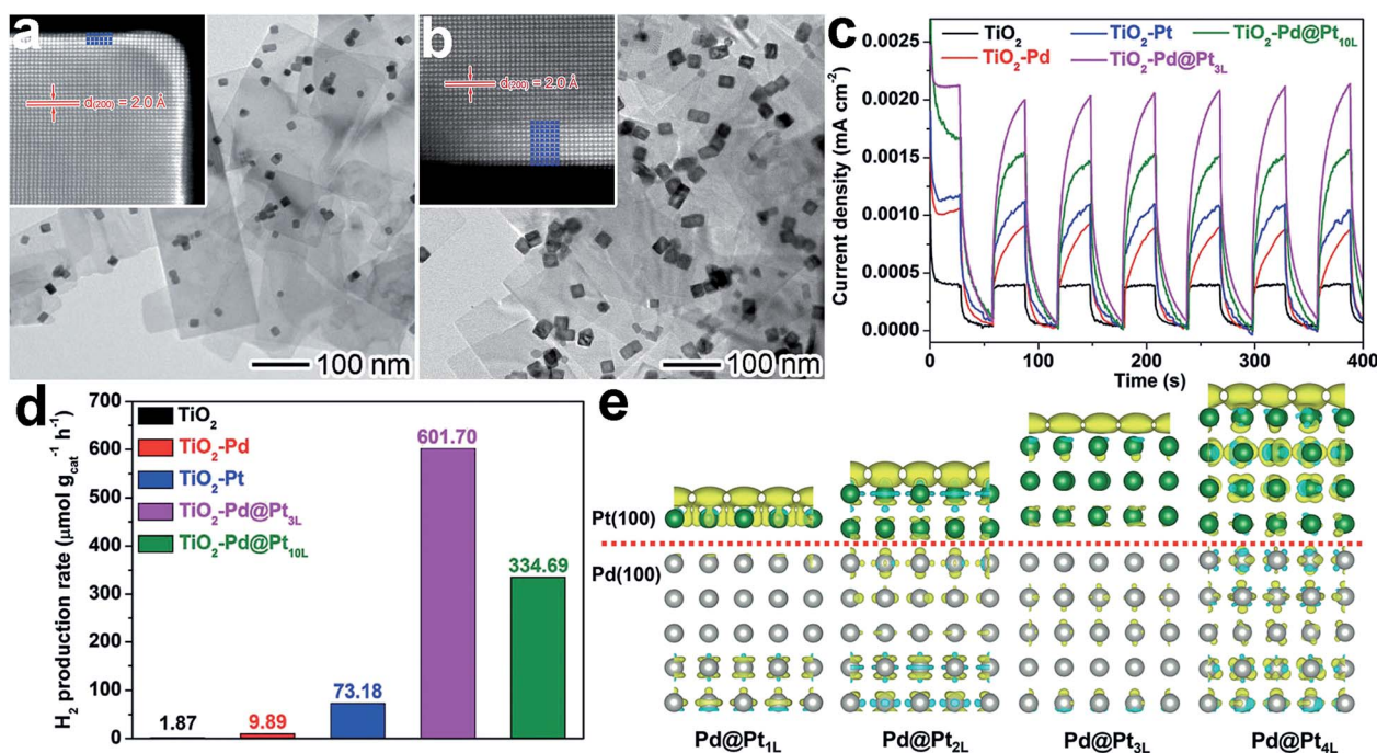
Fig. 12 (a and b) TEM images and atomic-resolution HAADF-STEM images of (a) Pd@Pt 3L and (b) Pd@Pt 10L quasi-core-shell cocatalysts supported on \text{TiO}_2 nanosheets; (c and d) I - t curves (c) and photocatalytic \text{H}_2 evolution (d) for \text{TiO}_2\text{-Pd@Pt}_{3\text{L}} and \text{TiO}_2\text{-Pd@Pt}_{10\text{L}} in comparison with bare \text{TiO}_2 nanosheets, \text{TiO}_2\text{-Pd} , and \text{TiO}_2\text{-Pt} hybrid structures under UV light irradiation; (e) differential charge density determined using first-principles simulations for Pt{100} shells on Pd{100} substrates in the presence of one additional electron: the olive and cyan colors represent an increase and decrease in electron density, respectively (adapted with permission from ref. 65, Copyright 2015 Wiley-VCH).
