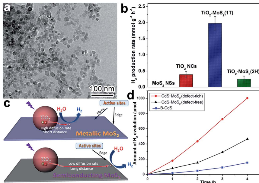
Fig. 6 (a) TEM image of \text{TiO}_2\text{-MoS}_2(1\text{T}) photocatalyst; (b) photocatalytic hydrogen production rates of \text{TiO}_2\text{-MoS}_2 ; (c) schematic diagram illustrating charge-transfer behavior and \text{H}_2 evolution active sites on \text{TiO}_2\text{-MoS}_2(1\text{T}) and \text{TiO}_2\text{-MoS}_2(2\text{H}) (adapted with permission from ref. 90, Copyright 2015 Springer); and (d) time course of \text{H}_2 evolution over CdS, CdS-MoS 2 (defect-free) and CdS-MoS 2 (defect-rich) (adapted with permission from ref. 91, Copyright 2015 Royal Society of Chemistry).
