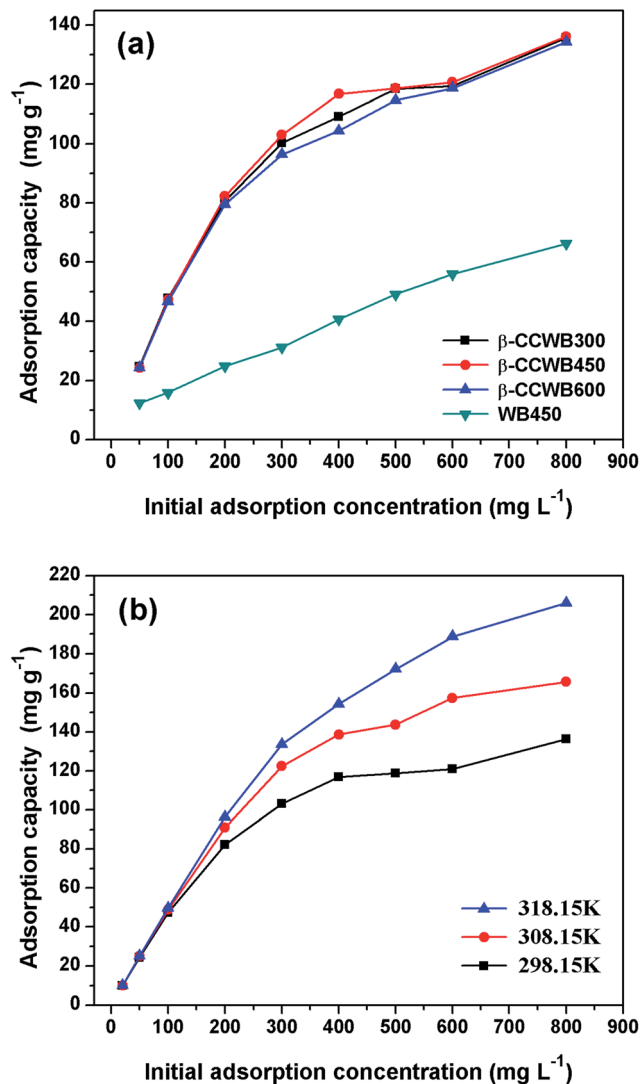
Fig. 4 (a) The comparison of adsorption capacity on \beta -CCWB and WB450 under 298.15 K, (b) the comparison of adsorption capacity on \beta -CCWB450 under different adsorption temperatures (Cr(vi) solution volume: 50 mL; adsorbent dose: 0.1 g; contact time: 24 h; pH: 2.0).
