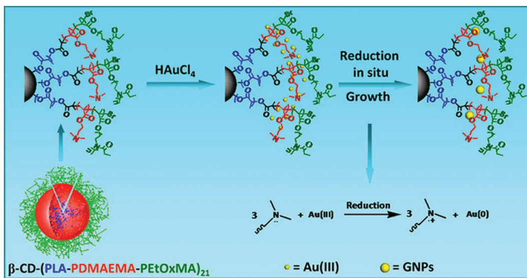
Fig. 19 Schematic representation of using the star-like block copolymer β-CD-(PLA-PDMAEMA-PtOxMA) 21 as a unimolecular micelle template for the synthesis and stabilization of gold nanoparticles. Reproduced with permission from Wiley. 201
