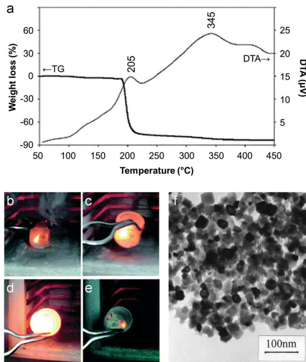
Fig. 4 (a) TGA/DTA trace for a mixture of citrate with barium and iron nitrates showing a sharp combustion at \sim 200 °C. (b–e) Images from a video of a combustion synthesis showing rapid progression of the reaction. (f) TEM image of a sample of a NiCuZn ferrite synthesized from a citrate/nitrate combustion method. Figures modified with permission from ref. 45, 46 and 48 respectively.
