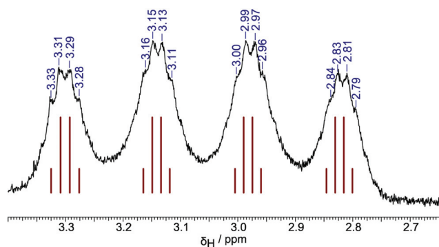
Fig. 3 Hydride resonance in 1 H NMR spectrum of Na[3-H], showing coupling to both 11 B ( I = 3/2) and an ortho -CF 3 group {3 × 19 F, I = 1/2}.
