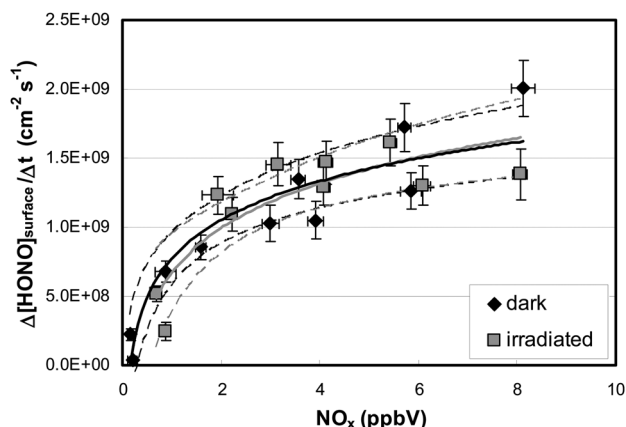
Fig. 6 HONO flux as a function of the NO x concentration calculated from the differences (dark-bypass) and (illuminated-bypass), ( [\text{HNO}_3]_{\text{surf}} \leq 0.8 \times 10^{14} \text{ cm}^{-2} , 51–54% r.h.). Within the experimental errors (95% confidence intervals, dashed lines), logarithmic fits (solid lines) show no difference between HONO formation in the dark (black) and under illumination (grey).
