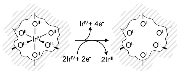
Fig. 4 \text{IrO}_6 octahedron in the near-surface region of the \text{IrO}_x framework (grey lines). Initially, Ir and O are in the formal oxidation states IV and II − , respectively. Upon the creation of an Ir vacancy, surrounding oxygen atoms are oxidized to the formal oxidation state I − . The two additional electrons are distributed among neighboring \text{Ir}^{\text{IV}} reducing them to \text{Ir}^{\text{III}} .
