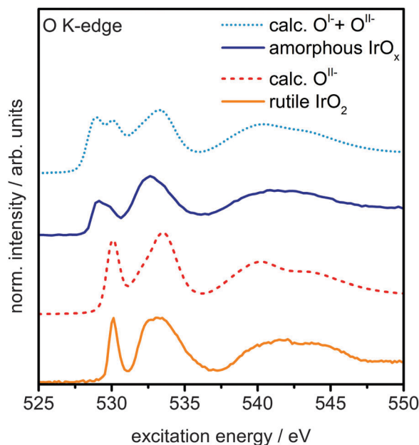
Fig. 3 Measured O K-edge spectra of rutile \text{IrO}_2 and amorphous \text{IrO}_x and calculated O K-edges of \text{O}^{\text{II-}} and a linear combination of 60% \text{O}^{\text{II-}} and 40% \text{O}^{\text{I-}} species.
