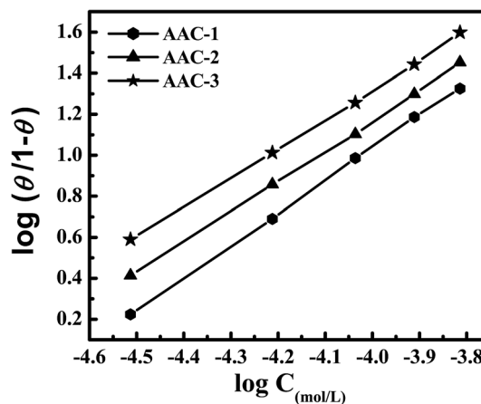
Fig. 4 Langmuir isotherm plots for the adsorption of AACs on mild steel surface in 1 M HCl.
